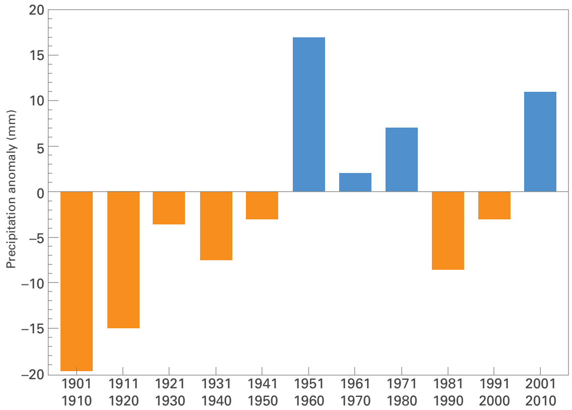
Figure 6. Decadal global precipitation anomaly (in mm) relative to the 1961–1990 WMO standard normal (source: NOAA-NCDC)
