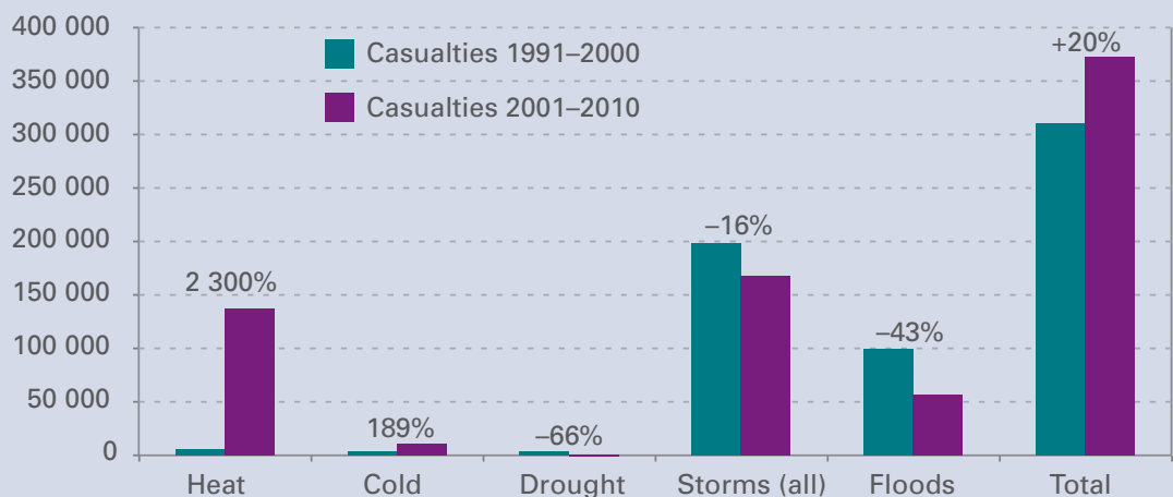
Figure 3. Impact of extreme events during 2001–2010 compared with 1991–2000: total number of lives lost. The change in per cent from 1991–2000 to 2001–2010 is shown above the bars. (data source: EM-DAT/CRED)
