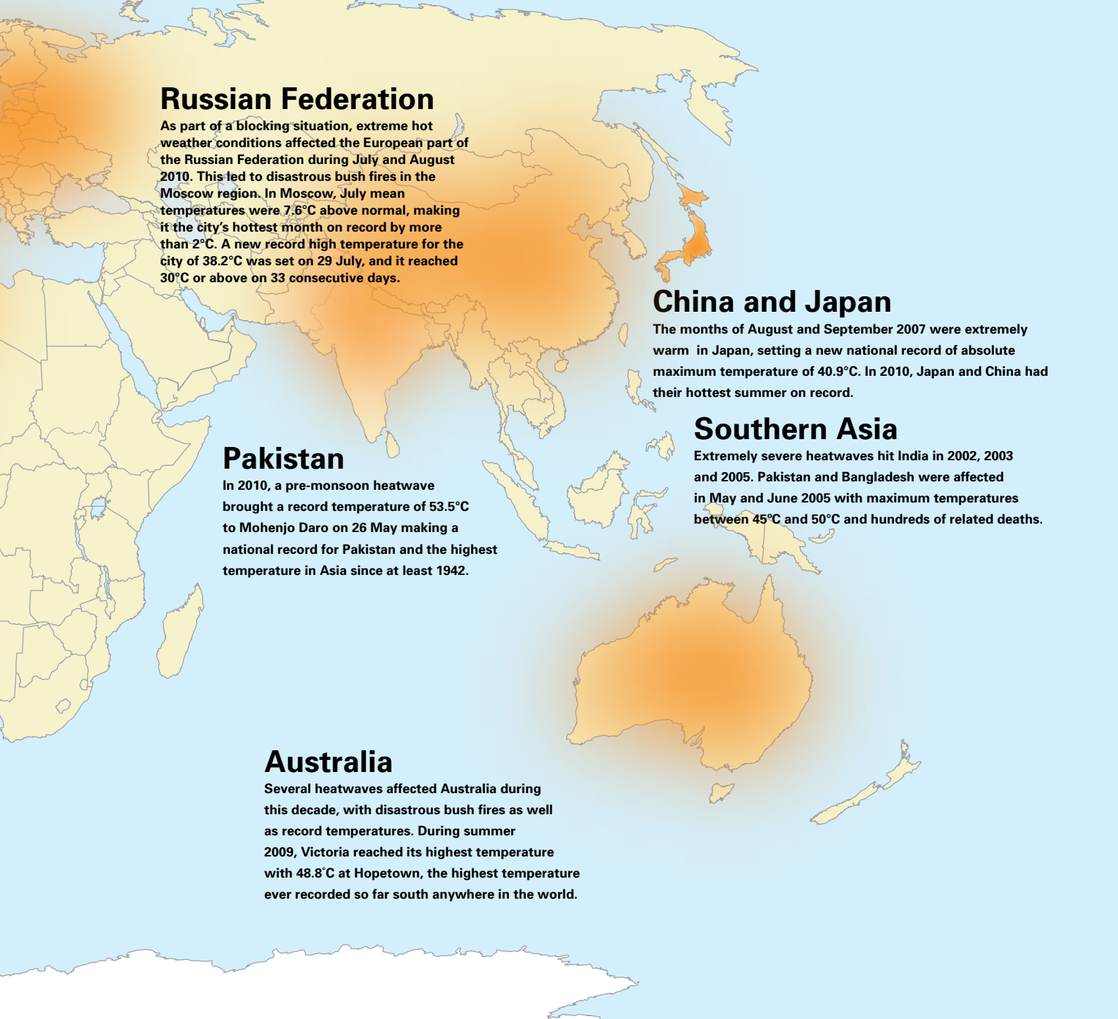
Figure 5. Most significant heatwaves and abnormally high temperature conditions reported during 2001–2010 (source: NOAA-NCDC)
