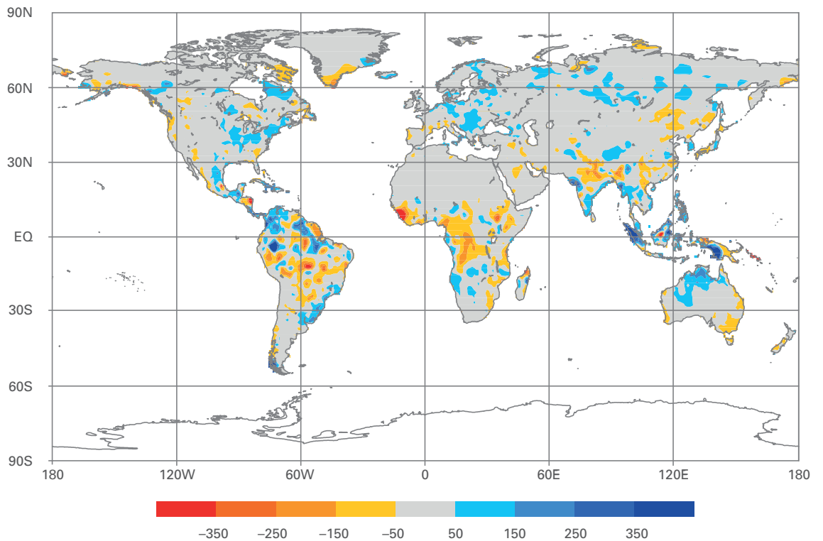
Figure 7. Decadal precipitation anomalies for global land areas for 2001–2010; gridded 1° raingauge-based analysis as normalized departures in mm/year focusing on 1951–2000 base period (source: Global Precipitation Climatology Centre (GPCC), Deutscher Wetterdienst, Germany)
