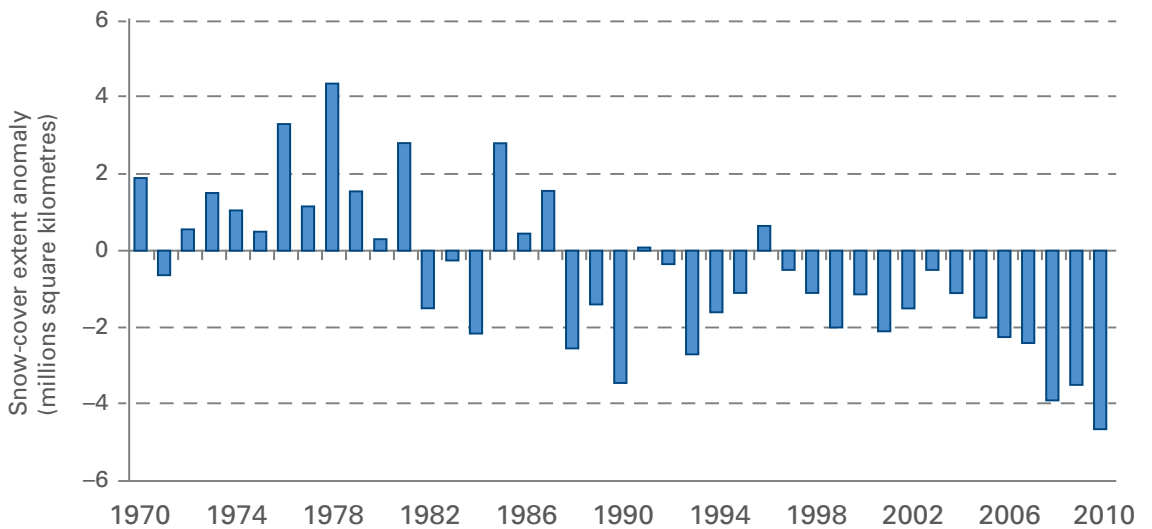
Figure 11. Northern hemisphere snow-cover anomaly for June (1970–2010) (data source: Rutgers University Global Snow Laboratory, USA).
