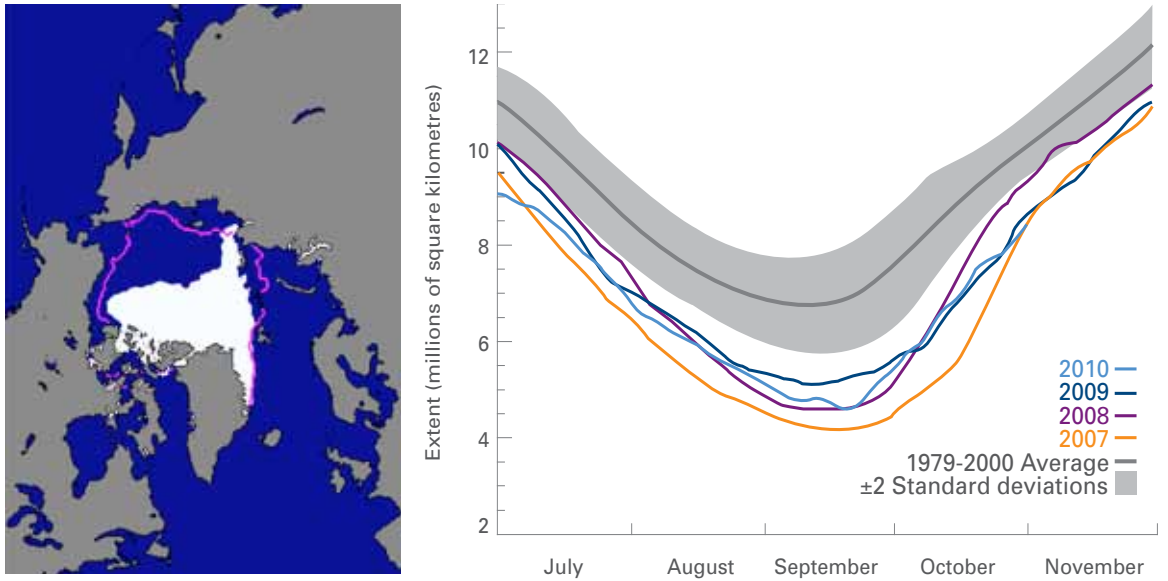
Figure 9. Sea-ice extent for September 2007; the magenta line indicates the long-term median from the 1979–2000 base period (left) and Arctic sea-ice extent at the end of the summer melt season from 2007 to 2010 (right) (source: National Snow and Ice Data Center, USA)
